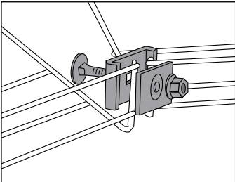
Horizontal bends are joined with Fitting B3.
