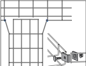
Four way and tees are joined with Fitting B3.
