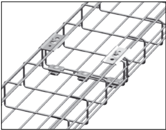
Joining of two C-Wire trays 220x80.
