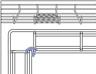
Wire tray 53 is shaped to straight 90° angle by cutting out marked wires and joined with Fitting B3.
