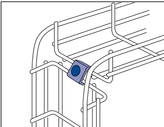
Vertical bends are joined with one or more Fitting B3, depending on wire tray width.
