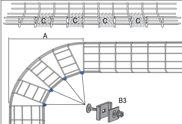
Wire tray 120-622 is shaped to straight 90 ° angle by cutting out every other marked wire tray section and joined with Fitting B3 according to table below.
